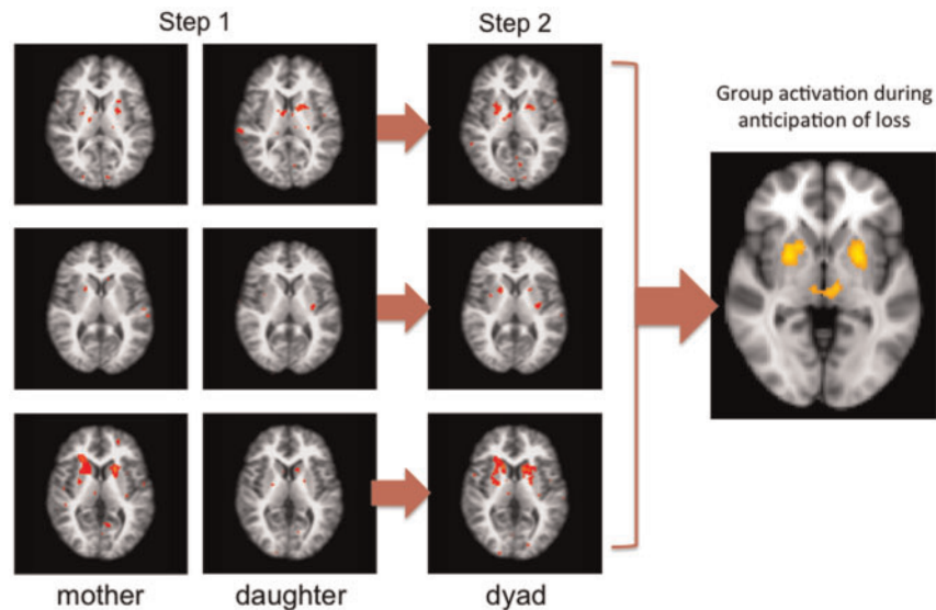
Fig. 1. We used a multistep analytic procedure to identify the association, or concordance, between mothers' and daughters' neural response to the anticipation of reward and loss. We first combined all participant-level data (from mothers and their daughters) into an average map for each dyad. We then combined all dyad maps to create a map of average activation for all participants for both anticipation of reward greater than neutral and anticipation of loss greater than neutral. Group Z-statistical maps for each condition (anticipation of reward and anticipation of loss) were thresholded at Z > 3.0 with a cluster probability of P < 0.01 , corrected for whole-brain multiple comparisons using Gaussian random field theory. We then isolated independent clusters of activation for each contrast across all participants and extracted parameter estimates (PEs) for both anticipation of reward vs anticipation of neutral and anticipation of loss vs anticipation of neutral for each individual.
